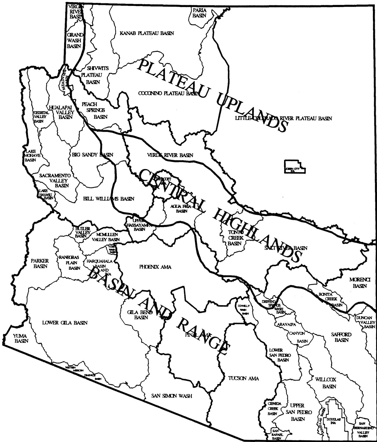
FIGURE 2 PHYSIOGRAPHIC PROVINCES OF ARIZONA
