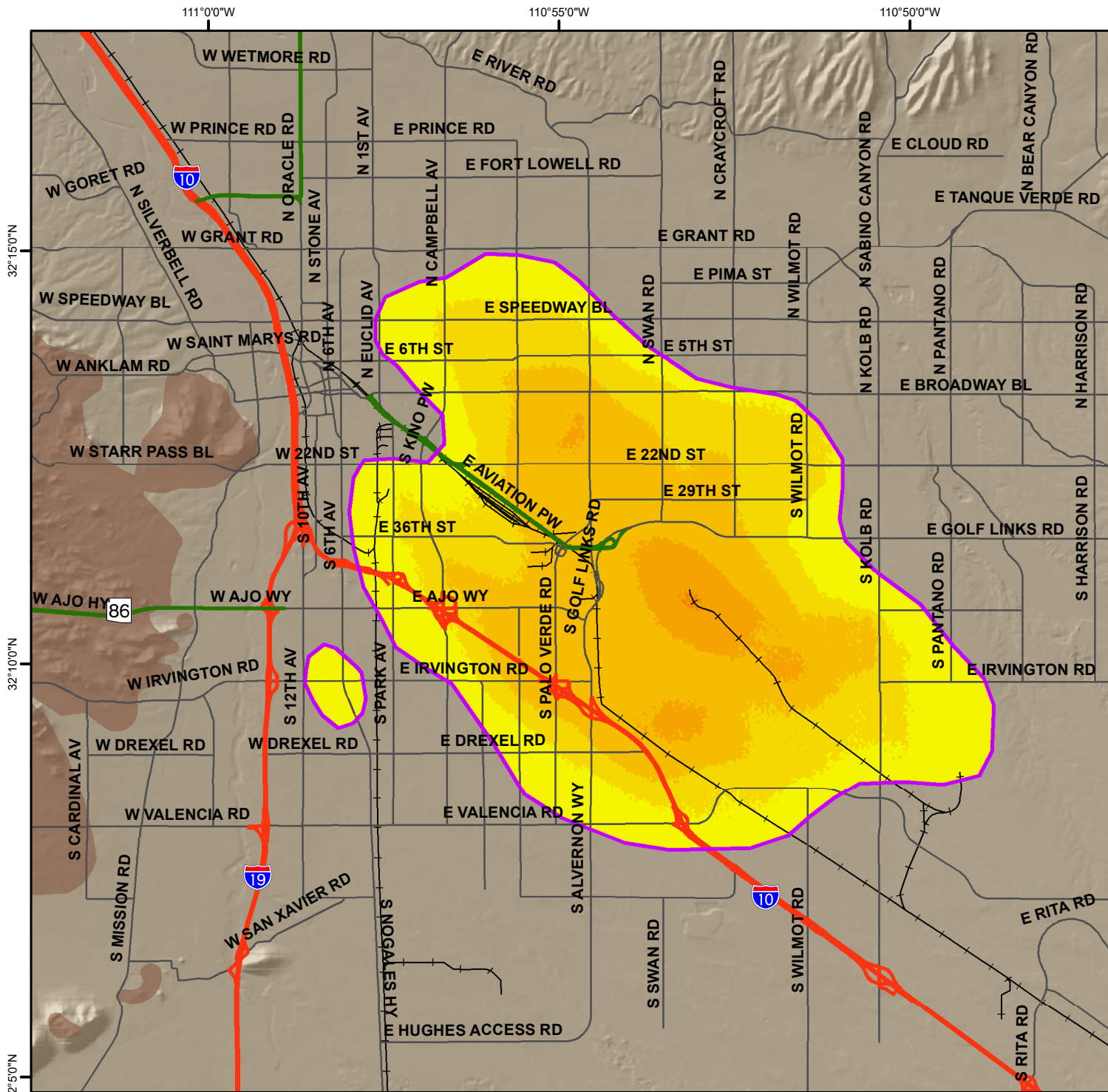
Total Land Subsidence in the Tucson Metropolitan Area Based on Radarsat-2 Satellite Interferometric Synthetic Aperture Radar (InSAR) Data Time Period of Analysis: 10.0 Years 05/15/2010 To 04/16/2020
