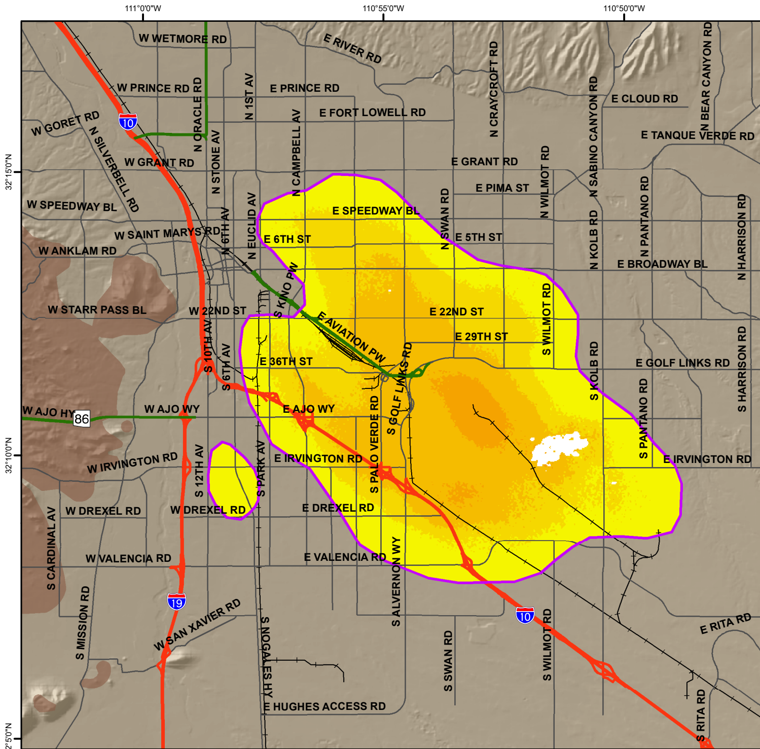
Total Land Subsidence in the Tucson Metropolitan Area Based on Radarsat-2 Satellite Interferometric Synthetic Aperture Radar (InSAR) Data Time Period of Analysis: 8.9 Years 05/15/2010 To 03/29/2019
