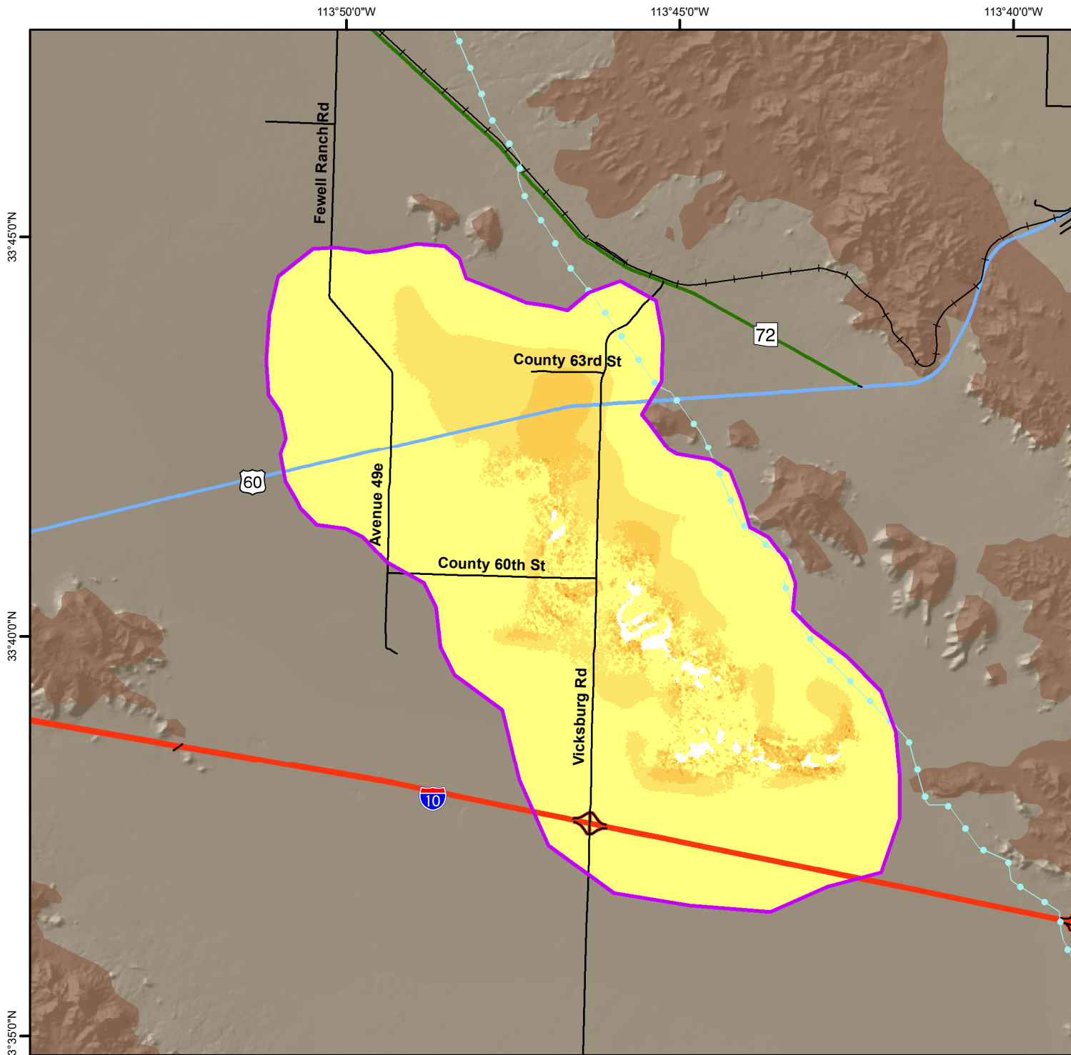
Land Subsidence Rate in the Ranegras Valley, La Paz County Based on Radarsat-2 Satellite Interferometric Synthetic Aperture Radar (InSAR) Data Time Period of Analysis: 1.0 Years 04/08/2019 To 04/26/2020
