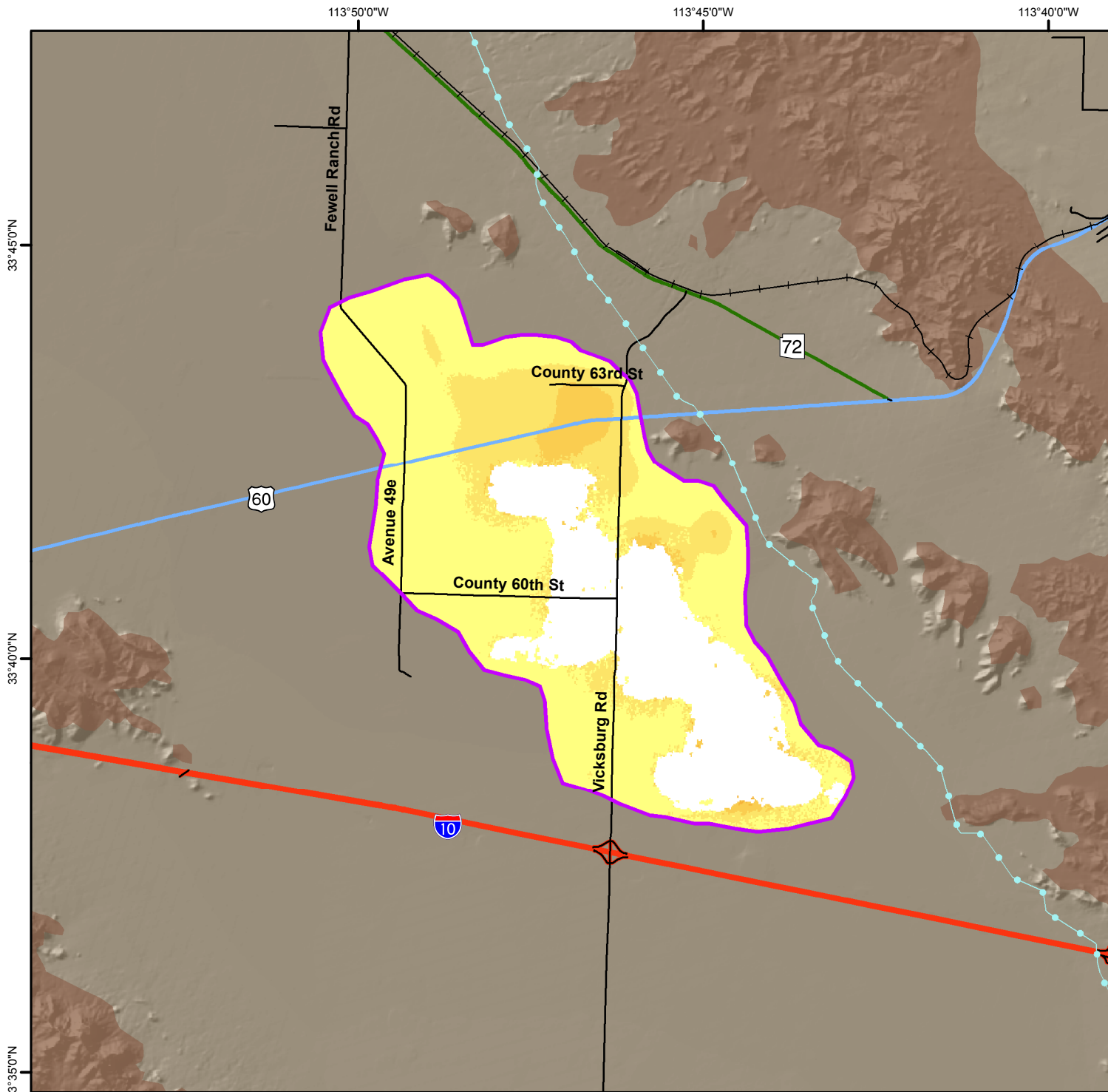
Land Subsidence Rate in the Ranegras Valley, La Paz County Based on Radarsat-2 Satellite Interferometric Synthetic Aperture Radar (InSAR) Data Time Period of Analysis: 1.0 Years 03/12/2015 To 03/30/2016
