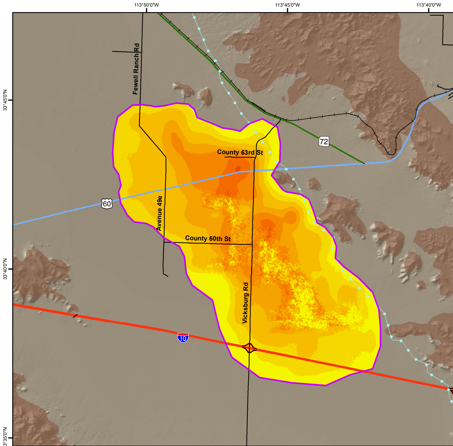
Total Land Subsidence in the Ranegras Valley, La Paz County Based on Radarsat-2 Satellite Interferometric Synthetic Aperture Radar (InSAR) Data Time Period of Analysis: 11.0 Years 05/01/2010 To 04/21/2021
