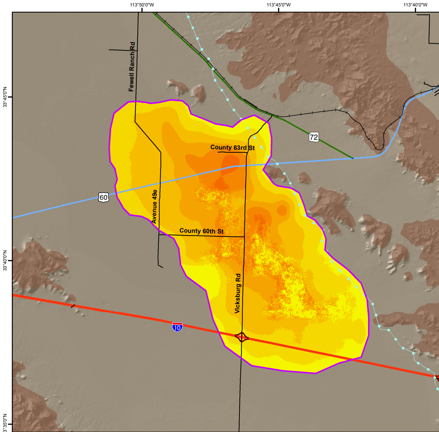
Total Land Subsidence in the Ranegras Valley, La Paz County Based on Radarsat-2 Satellite Interferometric Synthetic Aperture Radar (InSAR) Data Time Period of Analysis: 9.0 Years 05/01/2010 To 04/08/2019
