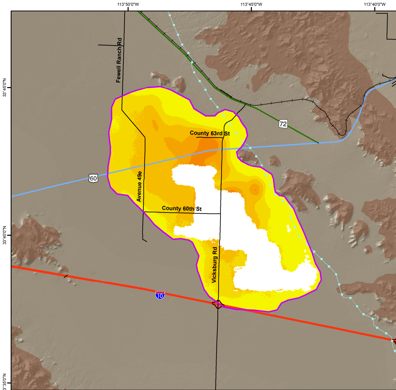
Total Land Subsidence in the Ranegras Valley, La Paz County Based on Radarsat-2 Satellite Interferometric Synthetic Aperture Radar (InSAR) Data Time Period of Analysis: 7.0 Years 05/01/2010 To 04/18/2017
