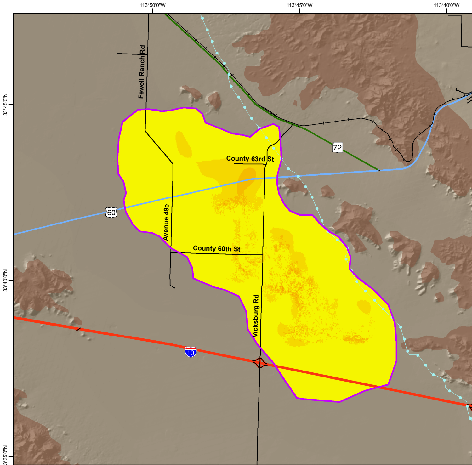
Total Land Subsidence in the Ranegras Valley, La Paz County Based on Radarsat-2 Satellite Interferometric Synthetic Aperture Radar (InSAR) Data Time Period of Analysis: 2.0 Years 04/08/2019 To 04/21/2021
