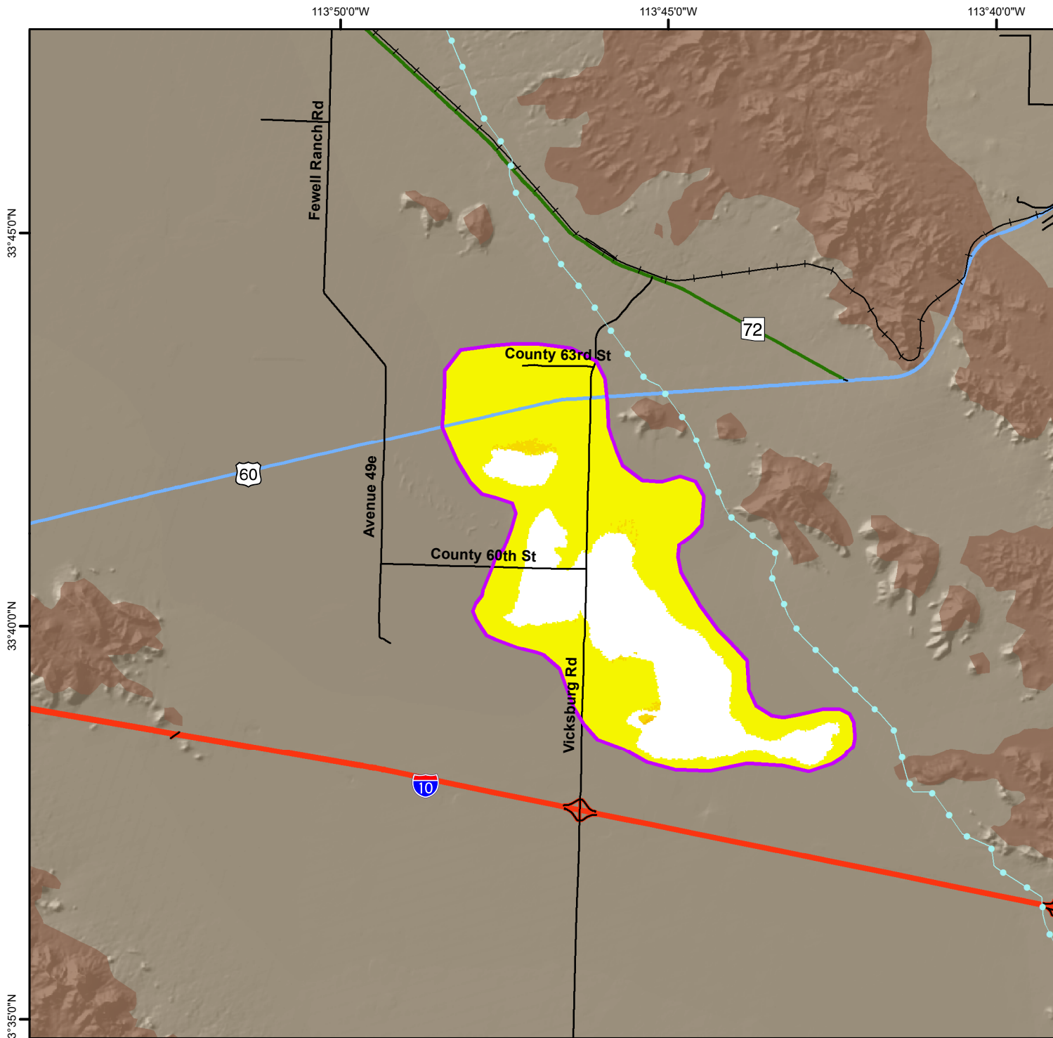
Total Land Subsidence in the Ranegras Valley, La Paz County Based on Radarsat-2 Satellite Interferometric Synthetic Aperture Radar (InSAR) Data Time Period of Analysis: 1.0 Years 04/18/2017 To 03/20/2018
