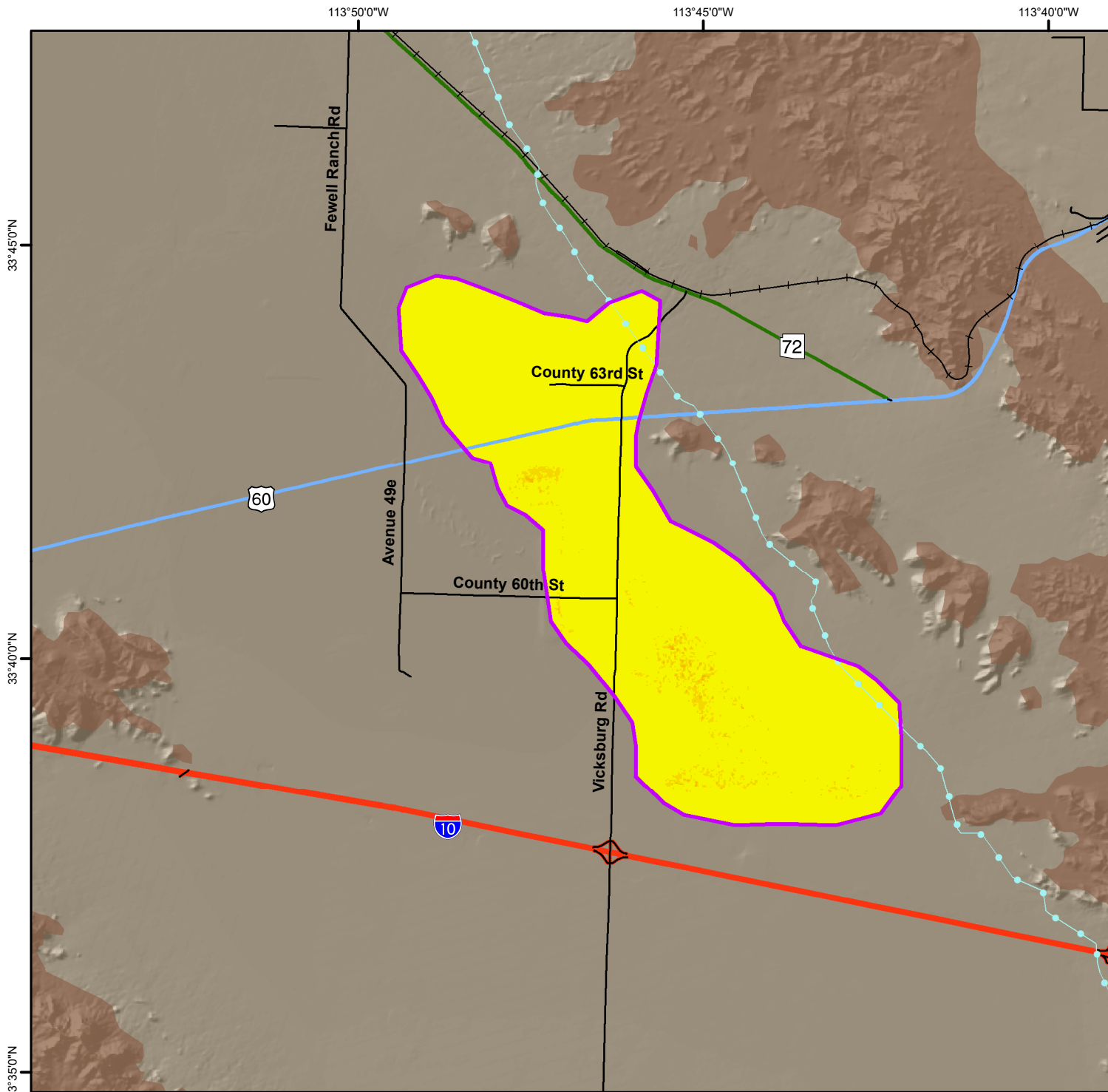
Total Land Subsidence in the Ranegras Valley, La Paz County Based on Radarsat-2 Satellite Interferometric Synthetic Aperture Radar (InSAR) Data Time Period of Analysis: 1.0 Years 03/09/2020 To 04/21/2021
