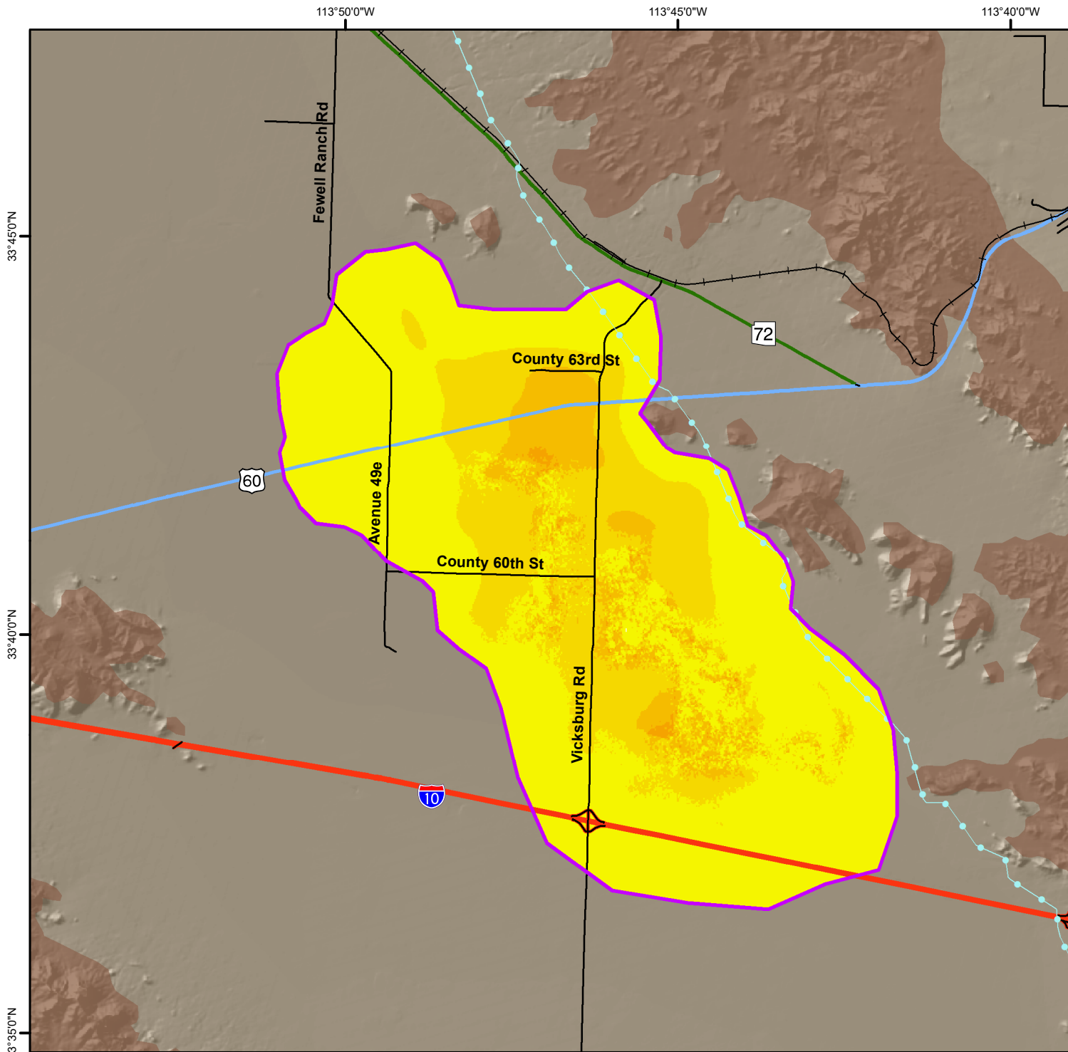
Total Land Subsidence in the Ranegras Valley, La Paz County Based on Radarsat-2 Satellite Interferometric Synthetic Aperture Radar (InSAR) Data Time Period of Analysis: 2.0 Years 03/25/2017 To 04/08/2019
