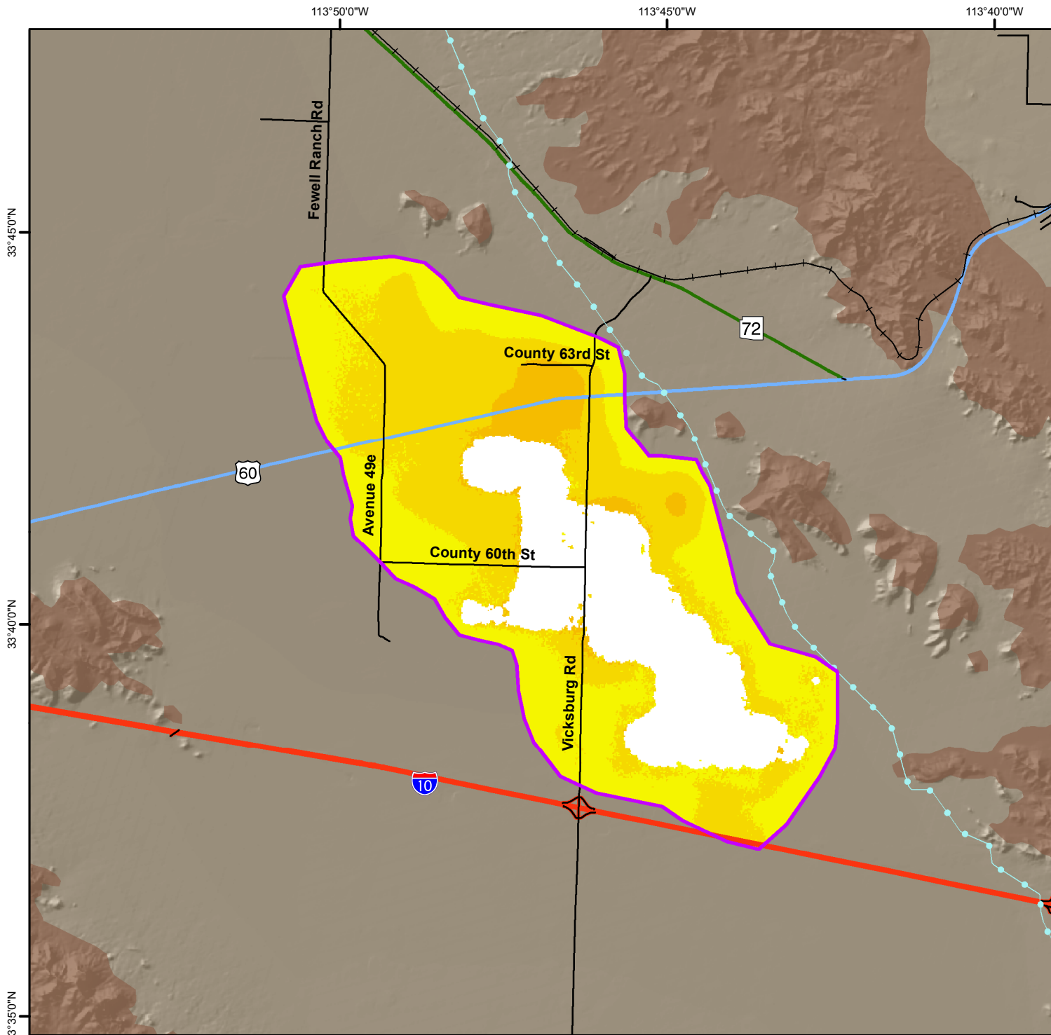
Total Land Subsidence in the Ranegras Valley, La Paz County Based on Radarsat-2 Satellite Interferometric Synthetic Aperture Radar (InSAR) Data Time Period of Analysis: 2.0 Years 03/17/2014 To 03/30/2016
