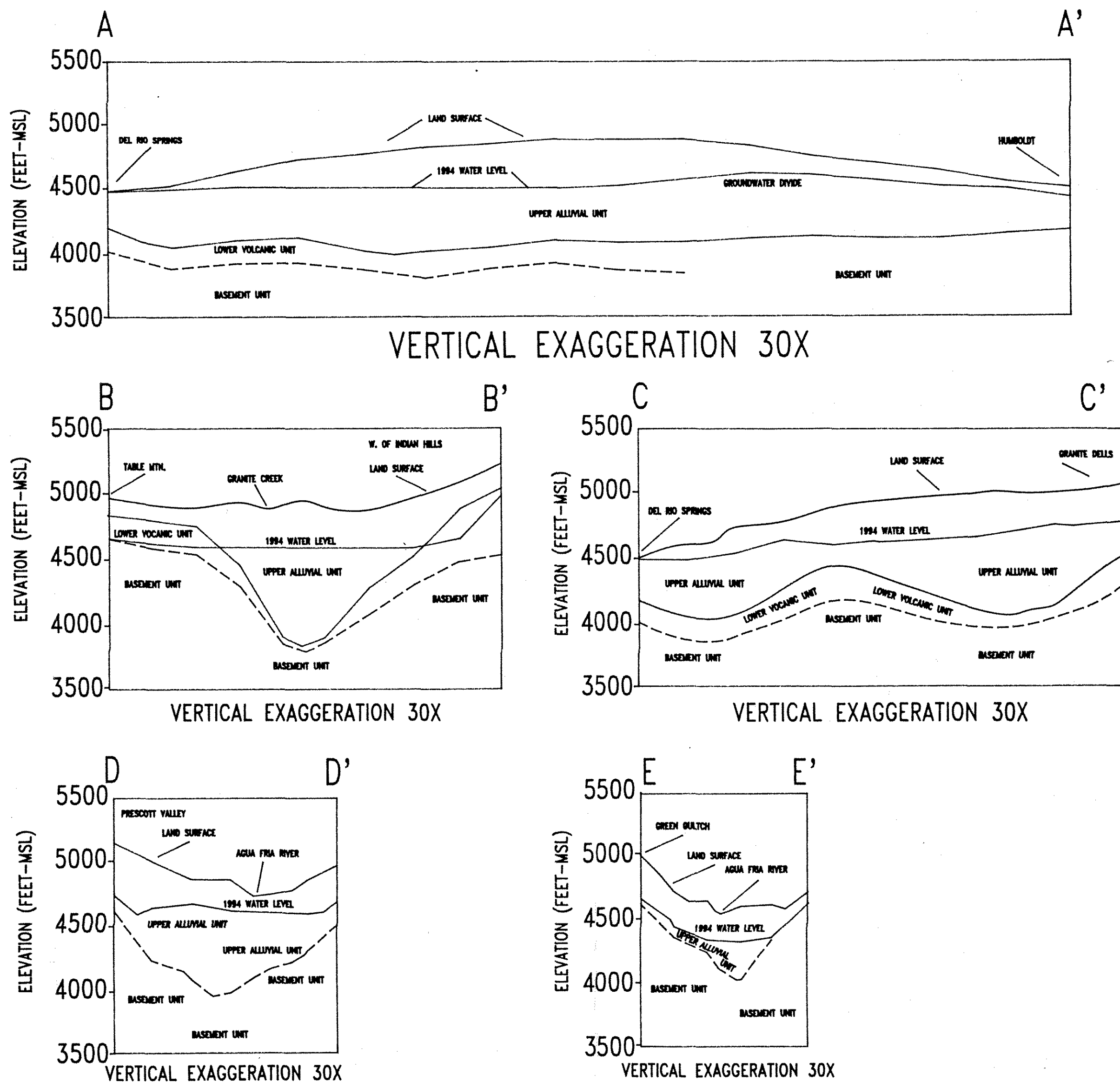
GENERALIZED HYDROGEOLOGIC CROSS-SECTIONS A-A' TO E-E'
