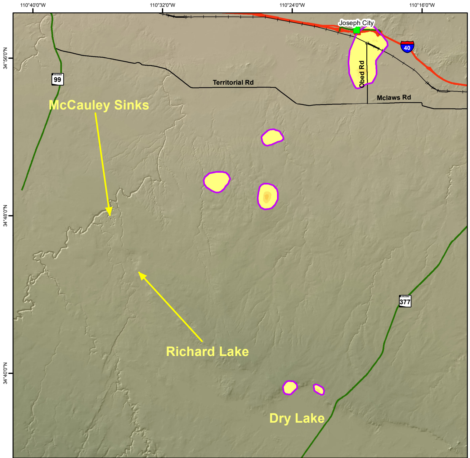
Land Subsidence Rate in the Holbrook Basin, Navajo County Based on Radarsat-2 Satellite Interferometric Synthetic Aperture Radar (InSAR) Data Time Period of Analysis: 7.6 Years 09/22/2012 To 05/31/2020
