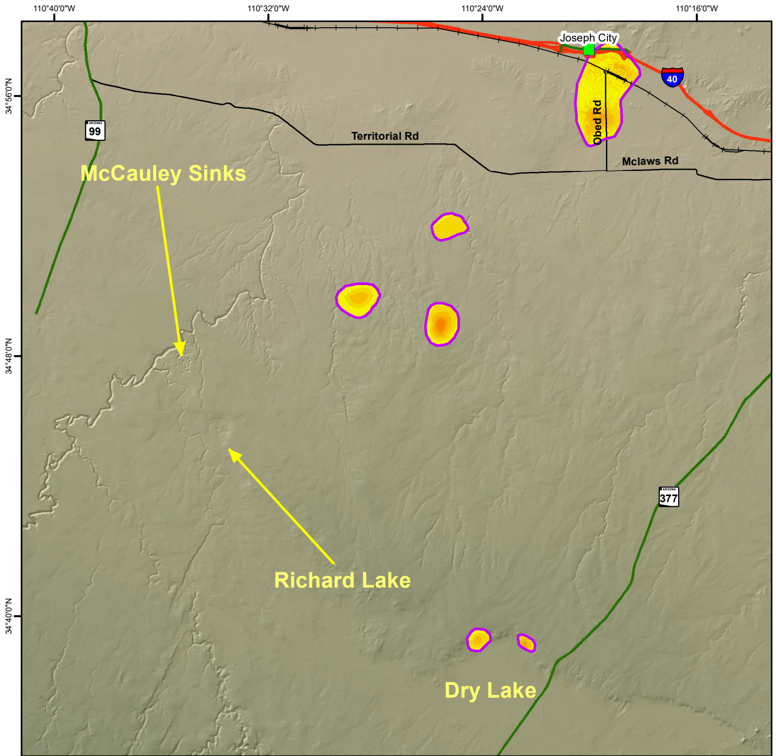
Total Land Subsidence in the Holbrook Basin, Navajo County Based on Radarsat-2 Satellite Interferometric Synthetic Aperture Radar (InSAR) Data Time Period of Analysis: 8.6 Years 09/22/2012 To 05/26/2021
