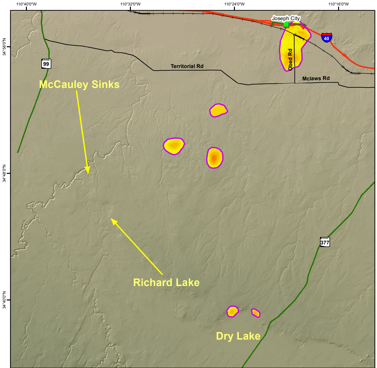
Total Land Subsidence in the Holbrook Basin, Navajo County Based on Radarsat-2 Satellite Interferometric Synthetic Aperture Radar (InSAR) Data Time Period of Analysis: 7.6 Years 09/22/2012 To 05/31/2020
