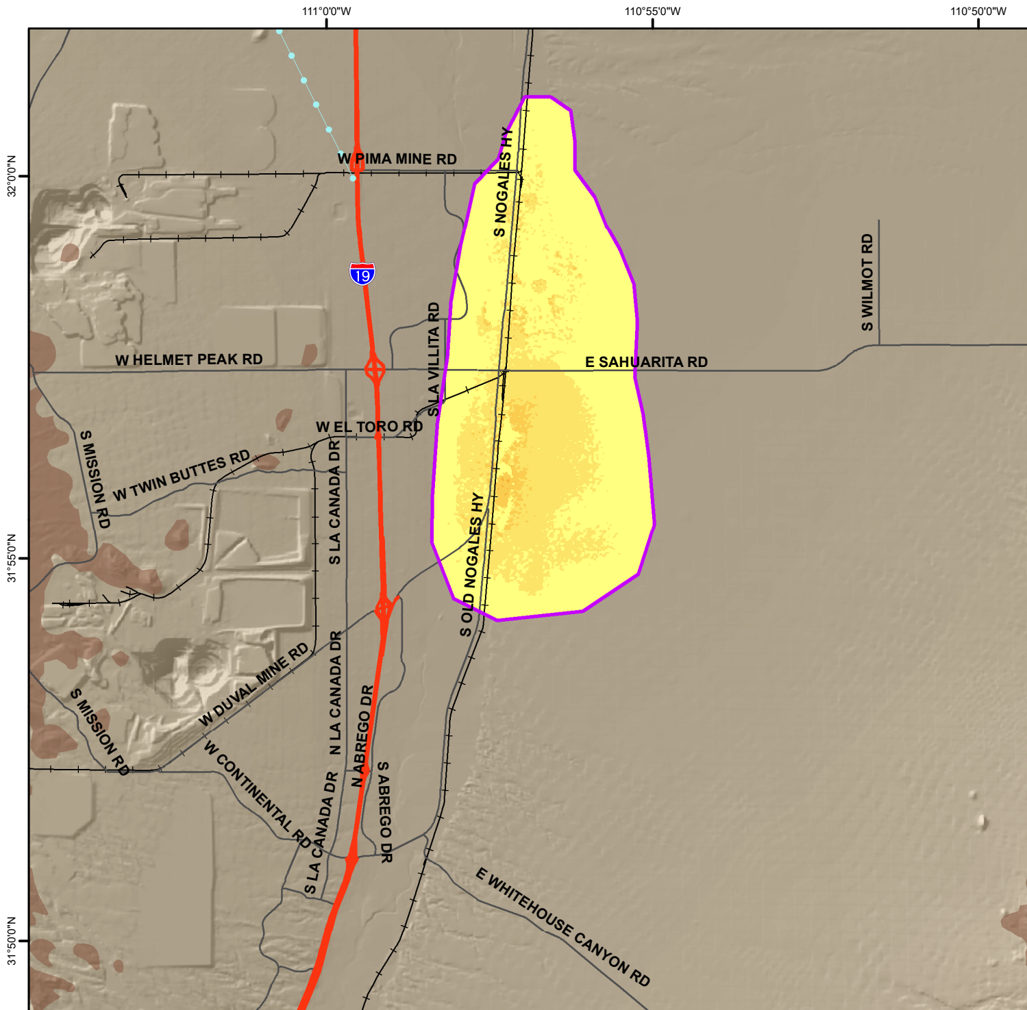
Land Subsidence Rate in the Sahuarita and Green Valley Areas, Pima County Based on Radarsat-2 Satellite Interferometric Synthetic Aperture Radar (InSAR) Data Time Period of Analysis: 2.1 Years 03/10/2018 To 04/16/2020
