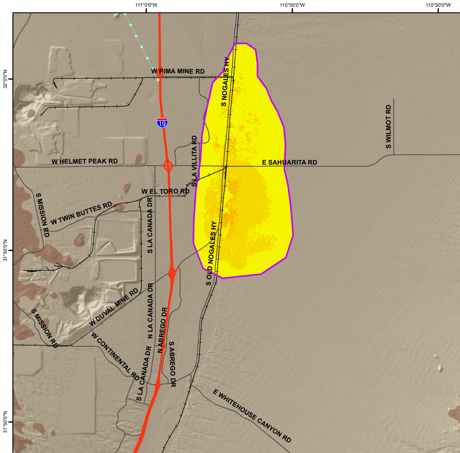
Total Land Subsidence in the Sahuarita and Green Valley Areas, Pima County Based on Radarsat-2 Satellite Interferometric Synthetic Aperture Radar (InSAR) Data Time Period of Analysis: 2.1 Years 03/10/2018 To 04/16/2020
