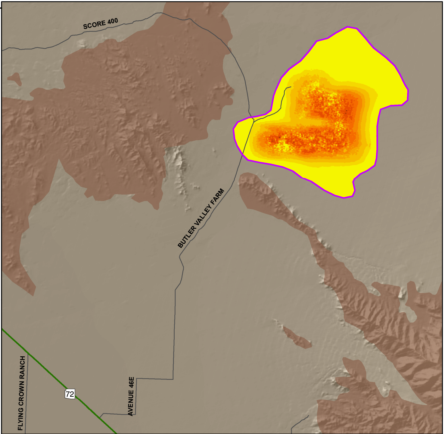
Land Subsidence in the Butler Valley Area, La Paz County Based on Sentinel-1 Satellite Interferometric Synthetic Aperture Radar (InSAR) Data Time Period of Analysis: 3.8 Years 04/23/2017 To 01/08/2021
