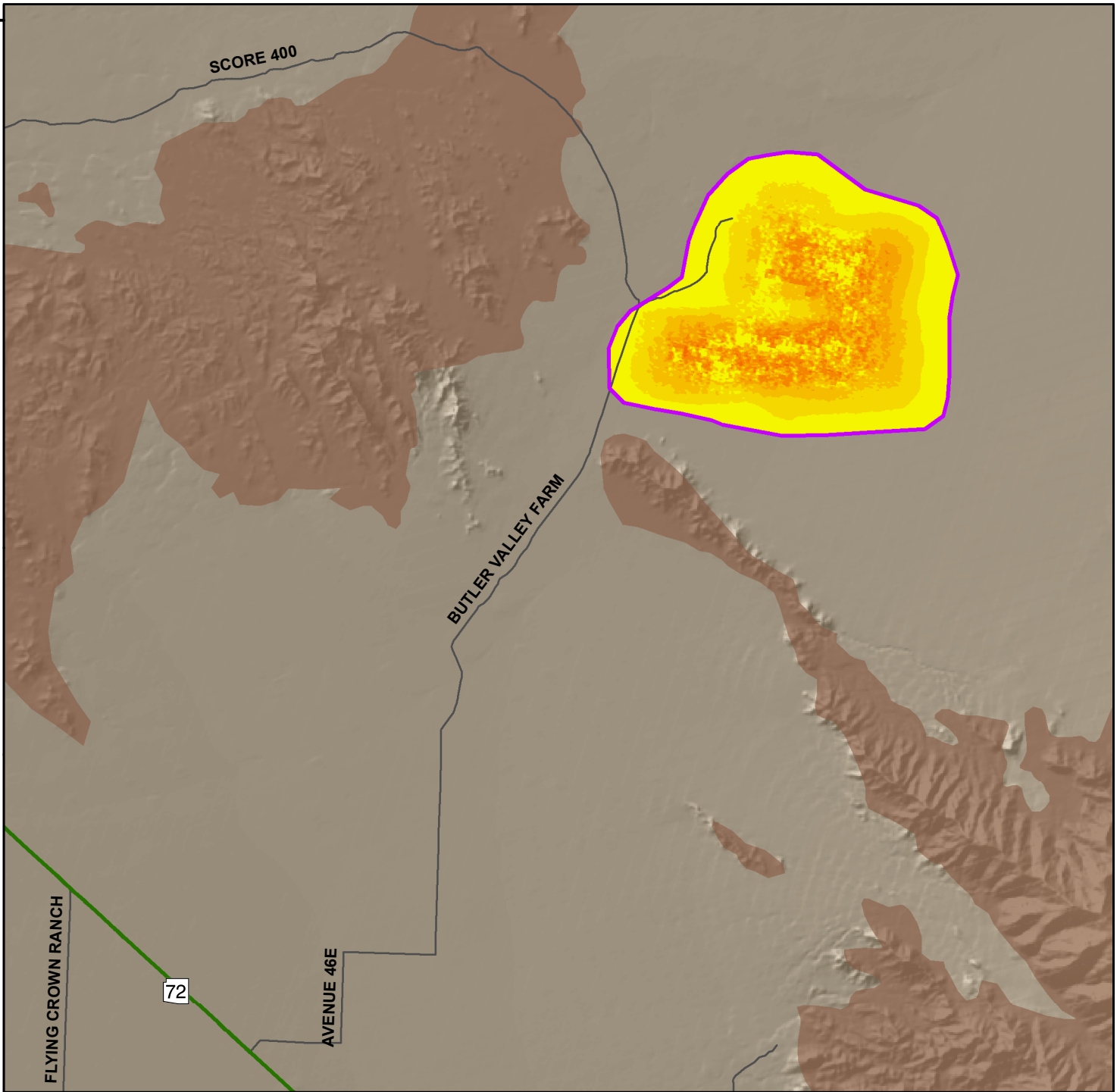
Land Subsidence in the Butler Valley Area, La Paz County Based on Sentinel-1 Satellite Interferometric Synthetic Aperture Radar (InSAR) Data Time Period of Analysis: 1.0 Years 02/12/2019 To 02/07/2020
